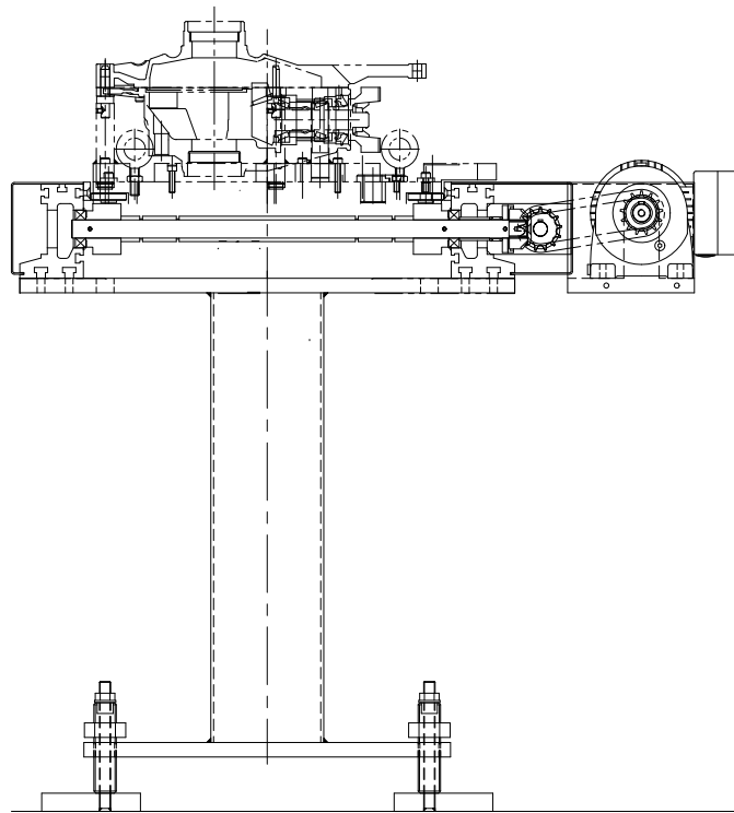
TYPICAL SECTION OF ROLLER CONVEYOR
